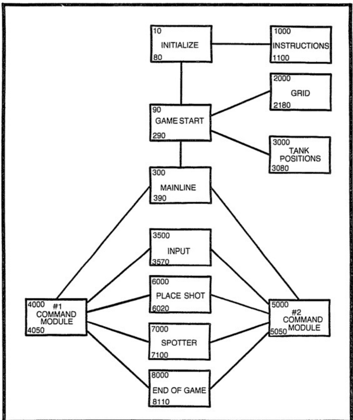
Fig. G-1. Program template for Gunners.
