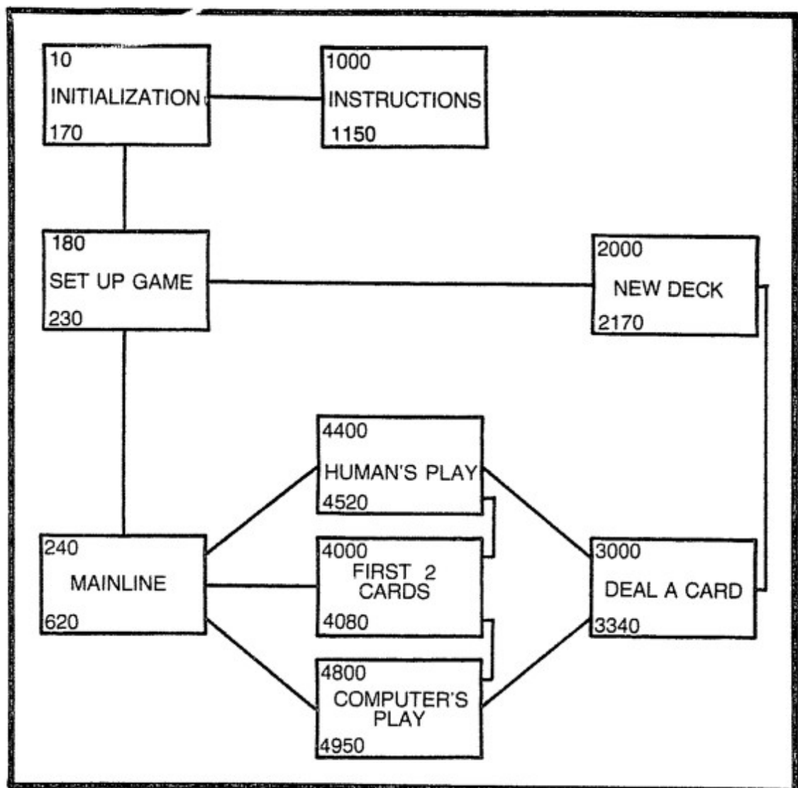
Fig. T-1. Program template for Twenty 1.
