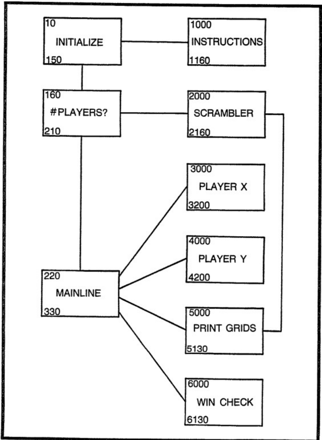
Fig. X-1. Program template for Xchange.
