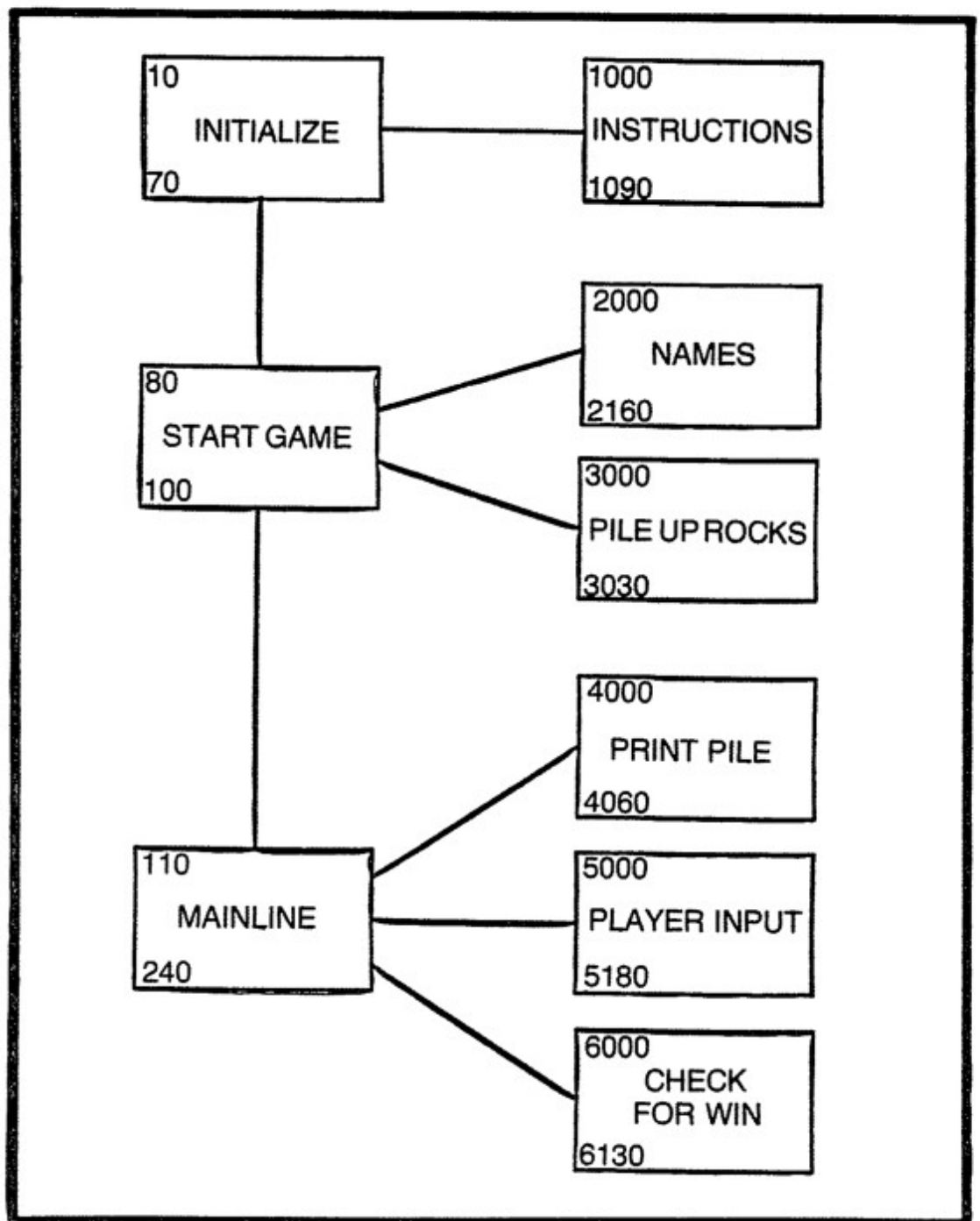
Fig. K-1. Program template for Knights.
