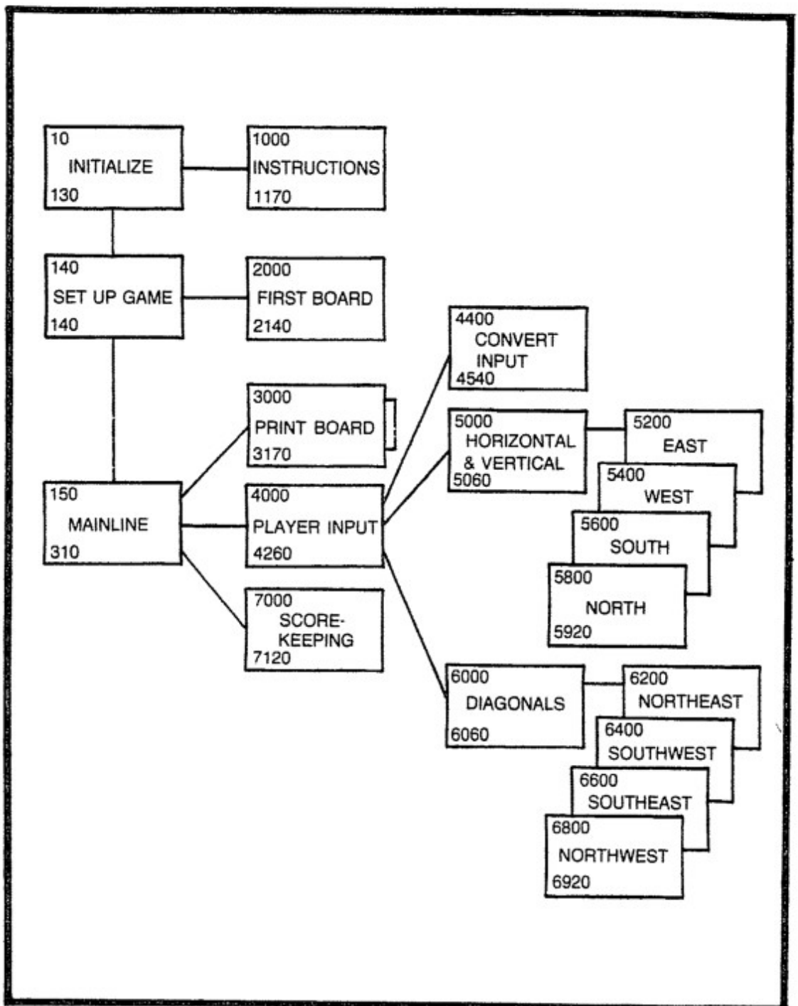
Fig. O-4. Program template for O-tell-O.
