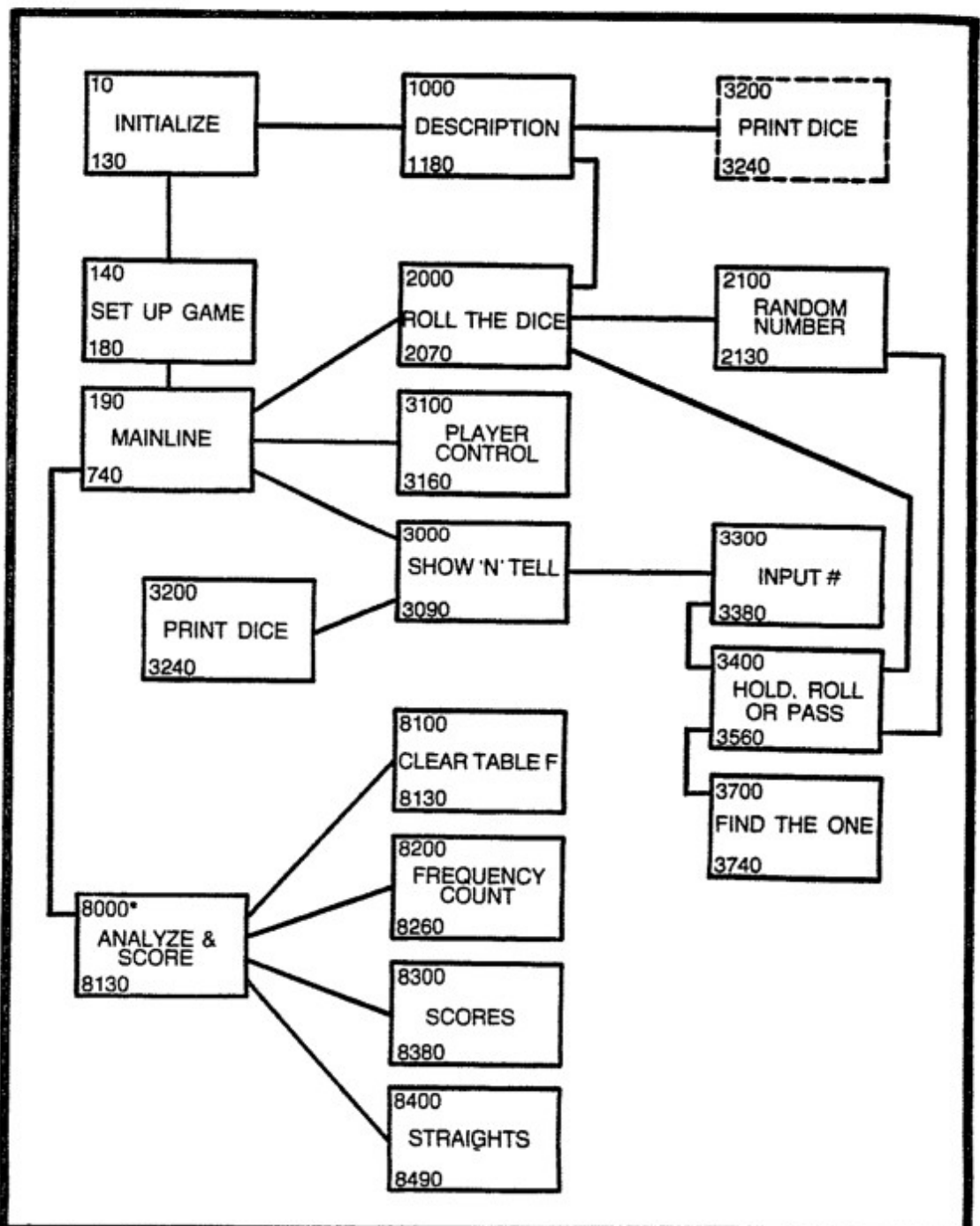
Fig. Y-1. Program template for Yat-C.
