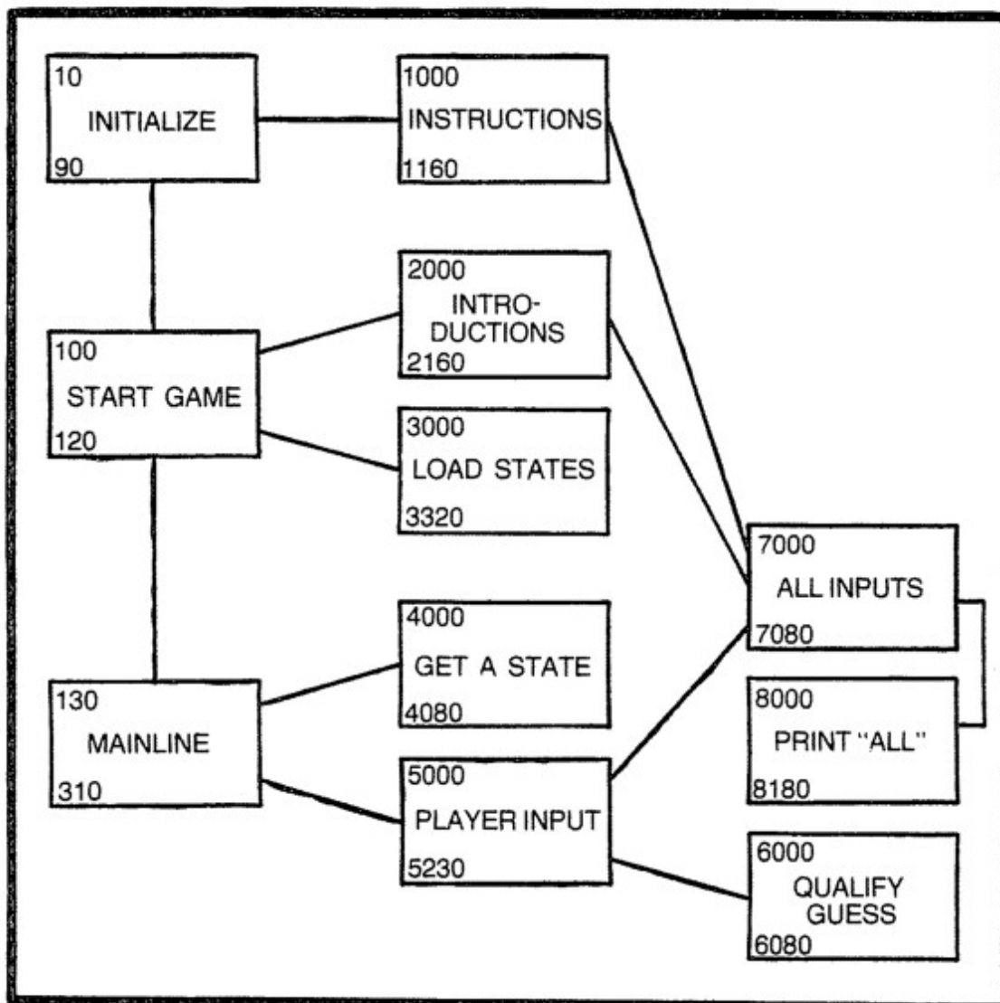
Fig. S-1. Program template for States.
