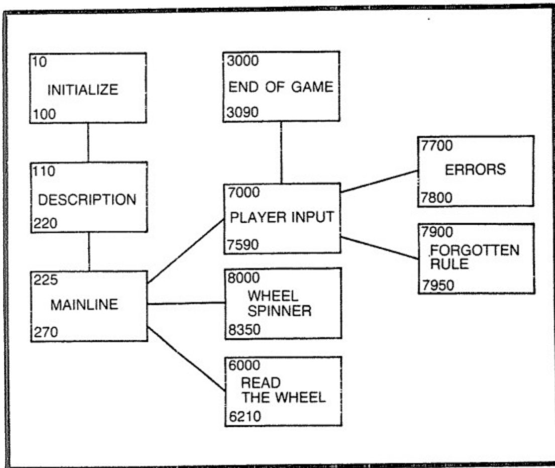
Fig. R-1. Program template for Roulette.
