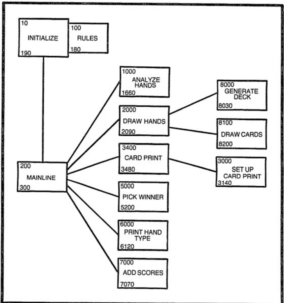
Fig. F-5. Program template for Fivecard.
