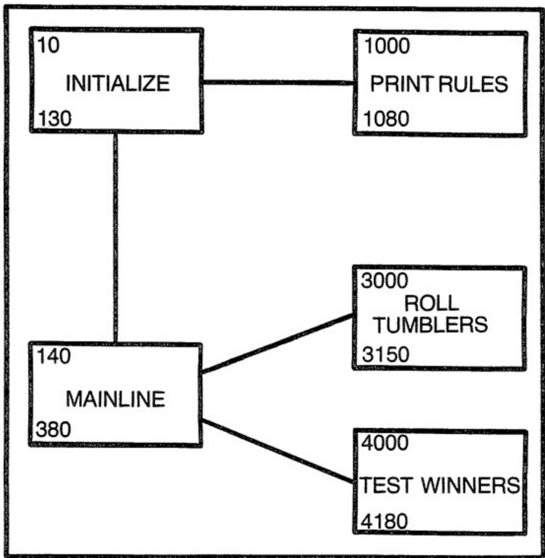
Fig. B-1. Program template for Bandit.
