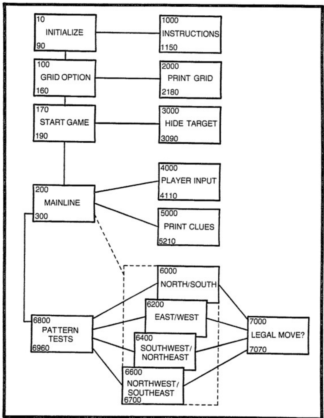
Fig. H-2. Program template for Hotshot.
