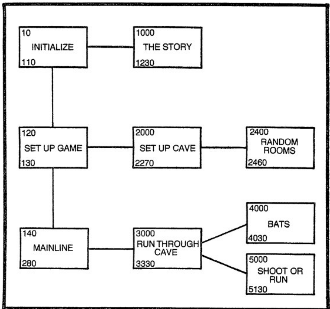
Fig. W-2. Program template for Wampus.
