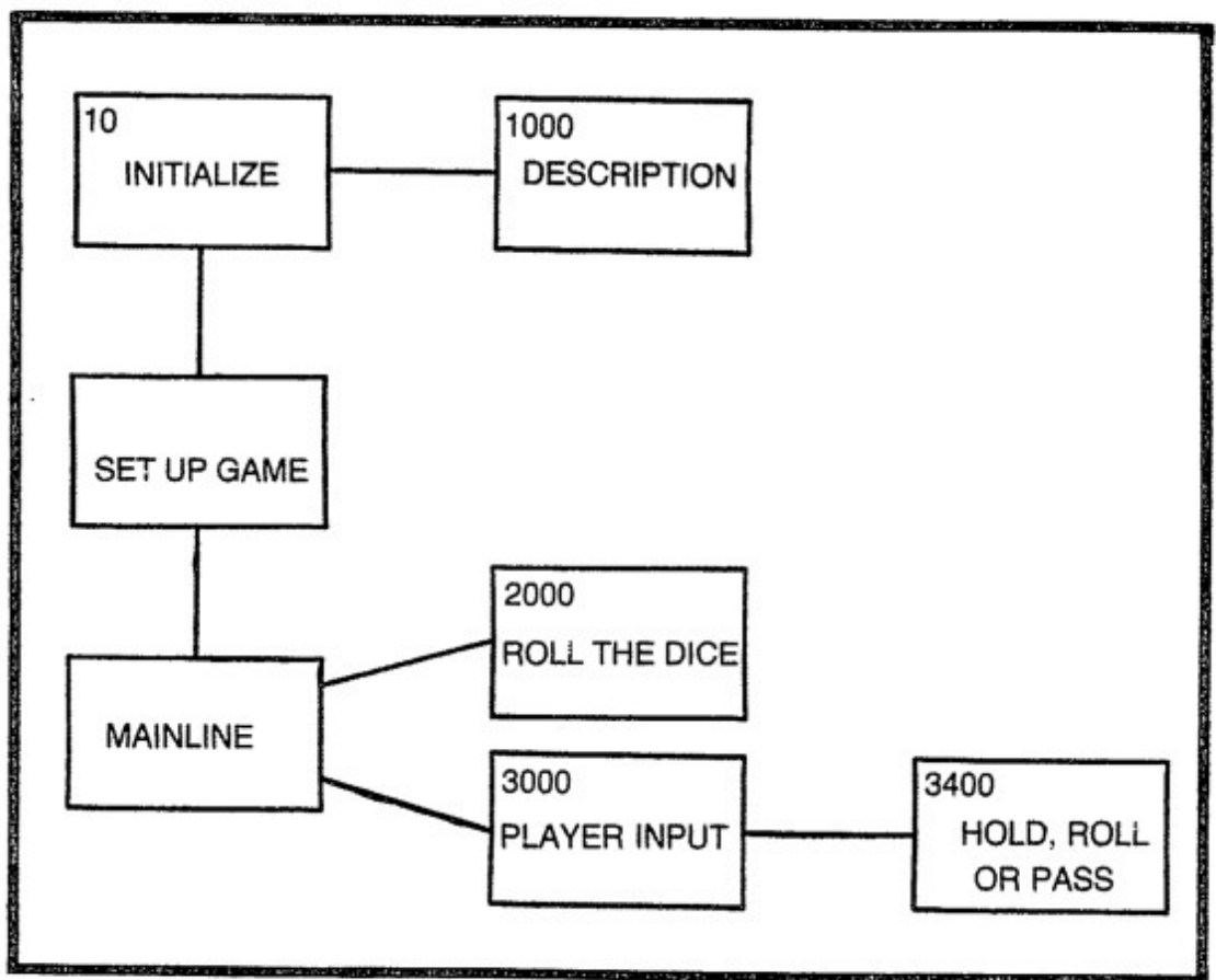
Fig. Y-2. The first-cut template for Yat-C.
