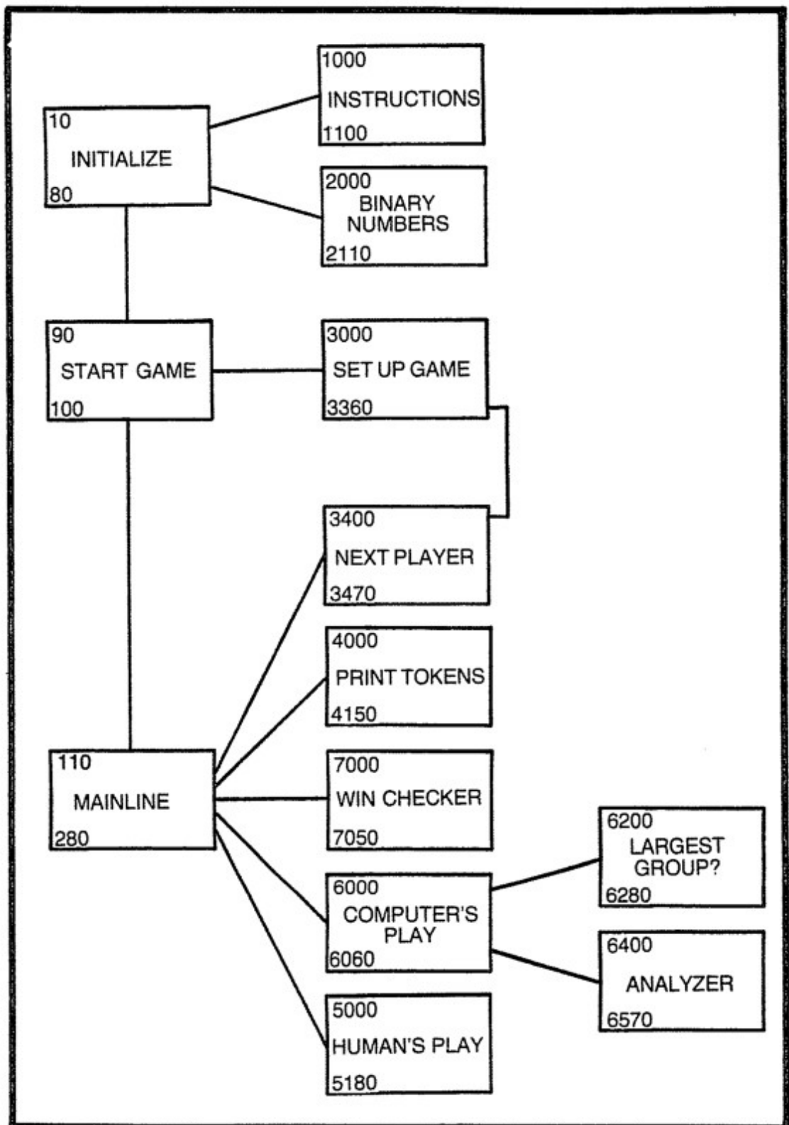
Fig. U-3. Program template for Ultranim.
