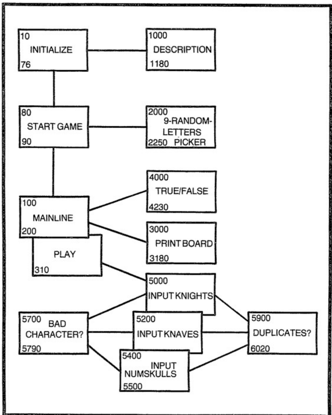
Fig. J-1. Program template for Justluck.
