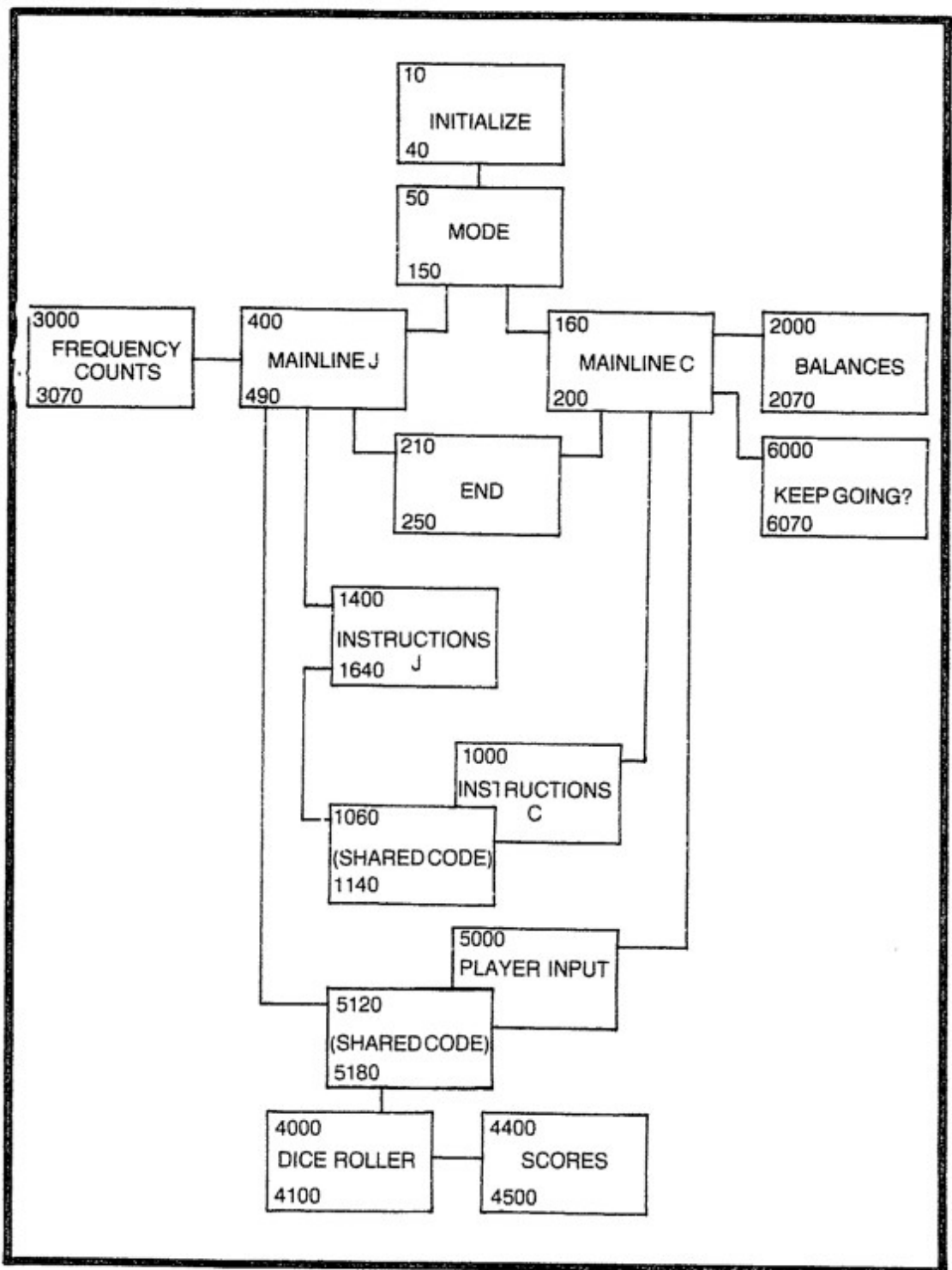
Fig. I-2. Program template for Invert.
