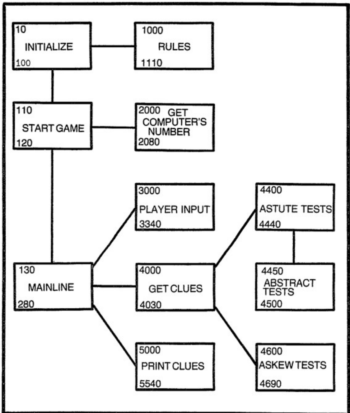
Fig. A-1. Program template for Abstract.
